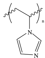
Poly(1-vinylimidazole)
